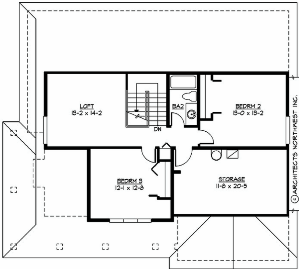
UPPER FLOOR PLAN
